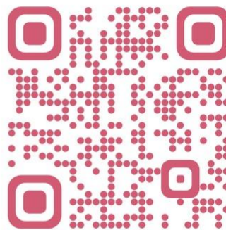
FCCmigex DATABASE
